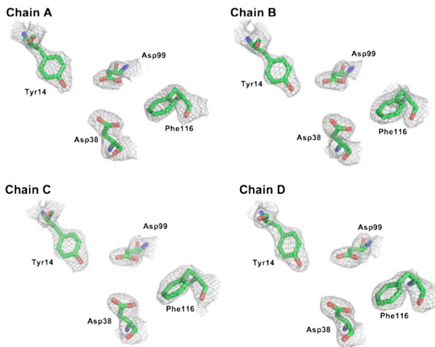
Fig. S1. 2F o -F c electron density map (contoured at 2.0σ) from the 2.5-Å resolution structure of Phe54Gly for the four independently refined chains contained in the asymmetric unit. Chain A has Asp38 indistinguishable from its position in wild-type ketosteroid isomerase (KSI), whereas the other three chains have Asp38 displaced ~1.0 Å from the wild-type KSI position.
