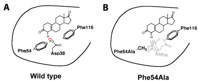
Fig. S3. Model for an increase in substrate binding for Phe54 mutants. (A) The anionic Asp general base is juxtaposed near to the hydrophobic steroid substrate in wild-type KSI, leading to an unfavorable interaction (red line). (B) Mutation of Phe54 to Ala, Gly, Val, and Ile allows the general base to access alternative conformations that reduce unfavorable interactions between the general base and steroid substrate leading to an increase in substrate binding (Fig. 3B).
