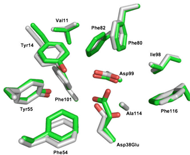
Fig. S2. Crystal structure of tKSI Asp38Glu shows that the base is mispositioned relative to wild-type tKSI. Superposition of the 2.1-Å Asp38Glu structure determined herein (PDB ID code 4L7K; carbon atoms are colored green) and the previously determined 2.3 Å wild-type KSI structure (PDB 8CHO; carbon atoms are color white). The overall root-mean-square deviation between the two structures for backbone atoms is 0.4 Å. X-ray data and refinement statistics are listed in Table S2.
